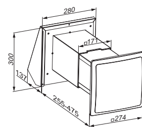
TwinFresh S-60 / SA-60
