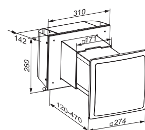
TwinFresh S-60-2 / SA-60-2
