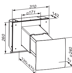
TwinFresh S1-50-2 / SA1-50-2
