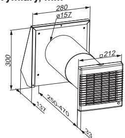
TwinFresh R-50 / RA-50
